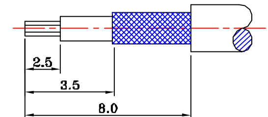
Recommended Cable Detail
