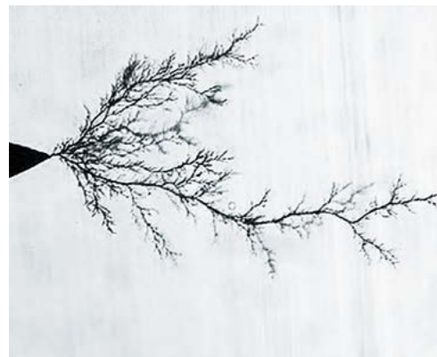
Typical effects on the insulator in the case of an incorrect connector layout: so-called "trees".
