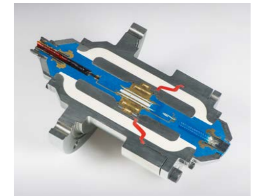
High-voltage feedthrough with connector for ITER – optimized and tested for freedom from partial discharge in all relevant areas.
