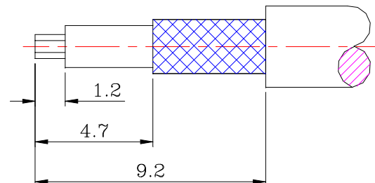
Recommended Cable Detail
