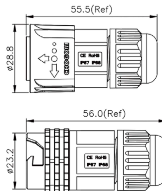
Field Installable Plug
