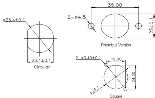
Panel Cut-Out(Circular & Square & Rhombus Version)
