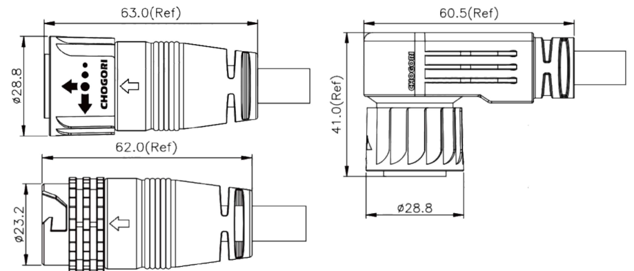
Overmold Plug(Straight & Right Angle Version)
