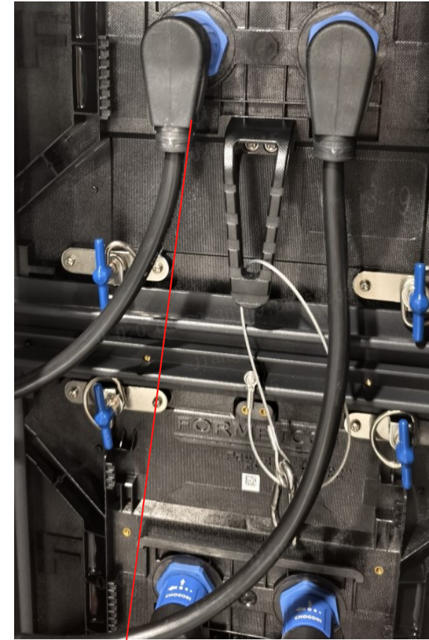
Middle 3P(20A)&8P(5A) Cable to Panel, Push Lock
