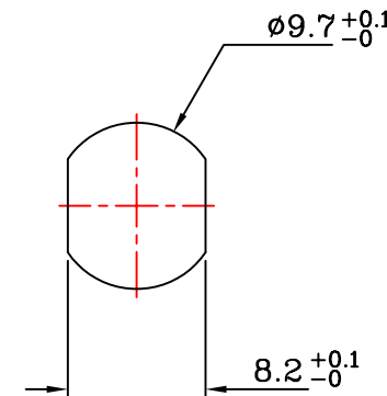
Recommended Panel Hole
