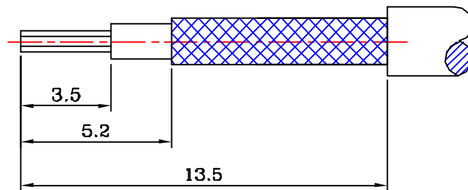
Recommended Cable Stripping Dim's
